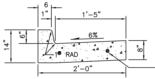
TYPICAL CURB AND GUTTER SECTION
