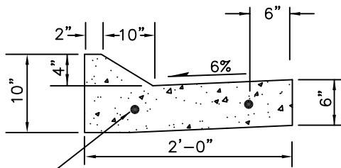
LIP CURB AND GUTTER SECTION
