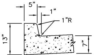
INTEGRAL UPRIGHT CURB SECTION AT 2% CROSS SLOPE
