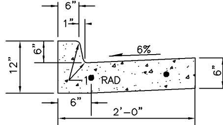
UPRIGHT CURB AND GUTTER SECTION
