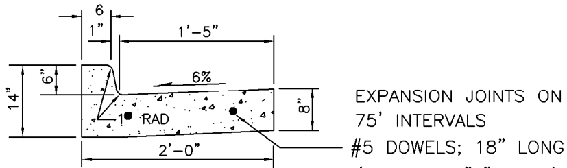
TYPICAL CURB AND GUTTER SECTION
