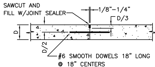
TYPE D (STREETS 7" AND GREATER) REINFORCED CONTRACTION JOINT
