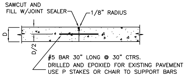
TYPE L LONGITUDINAL CONSTRUCTION JOINT (With Steel)
