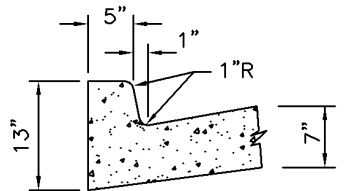
INTEGRAL UPRIGHT CURB SECTION AT 6% CROSS SLOPE
