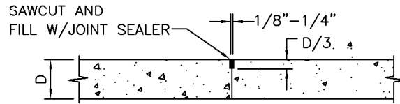
TYPE C (WITHOUT TIE BAR) CONTRACTION JOINT
