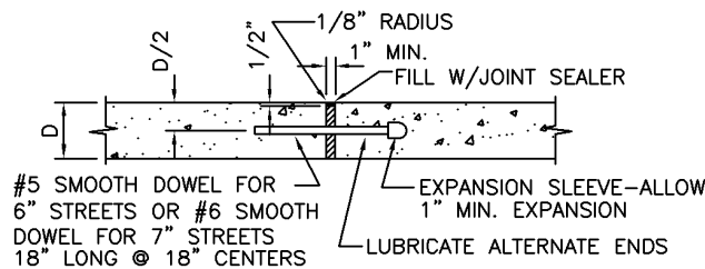
TYPE E REINFORCED EXPANSION JOINT
