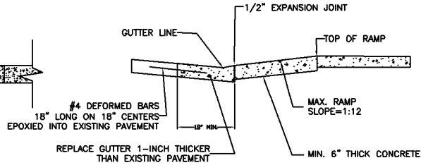
TYPICAL PROFILE NTS
