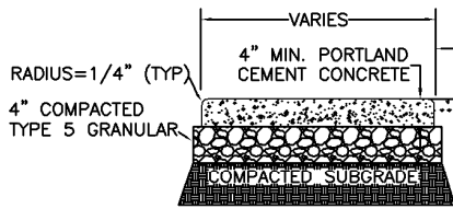
CROSS SECTIONAL VIEW NTS
