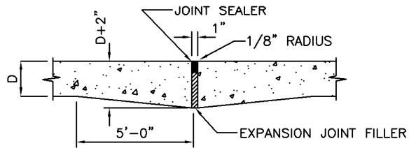
TYPE A EXPANSION JOINT OR PAVEMENT TERMINATION
