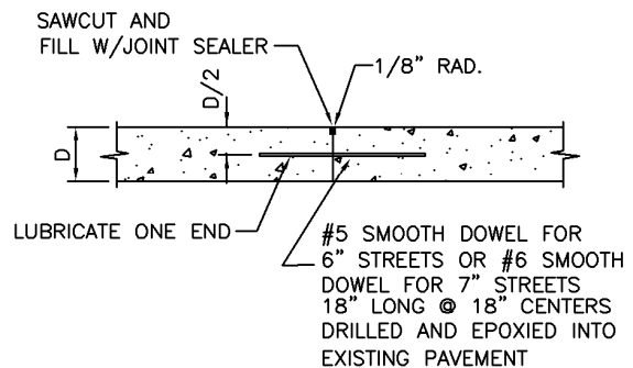
TYPE B TRANSVERSE CONSTRUCTION JOINT
