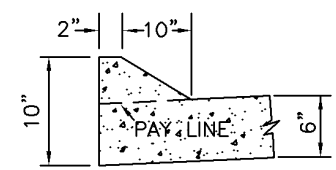
INTEGRAL LIP-TYPE CURB SECTION
