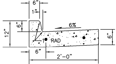
UPRIGHT CURB AND GUTTER SECTION
