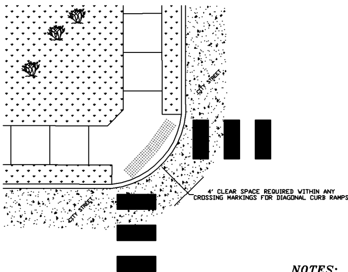
PLAN VIEW SINGLE DOWN SET RAMP SIDEWALK OFFSET FROM CURB
