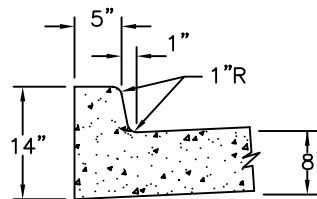
INTEGRAL UPRIGHT CURB SECTION
