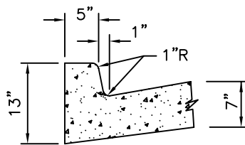
INTEGRAL UPRIGHT CURB SECTION AT 6% CROSS SLOPE
