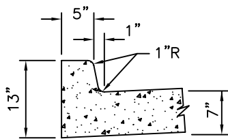
INTEGRAL UPRIGHT CURB SECTION AT 2% CROSS SLOPE
