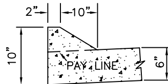
INTEGRAL LIP-TYPE CURB SECTION
