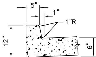
INTEGRAL UPRIGHT CURB SECTION
